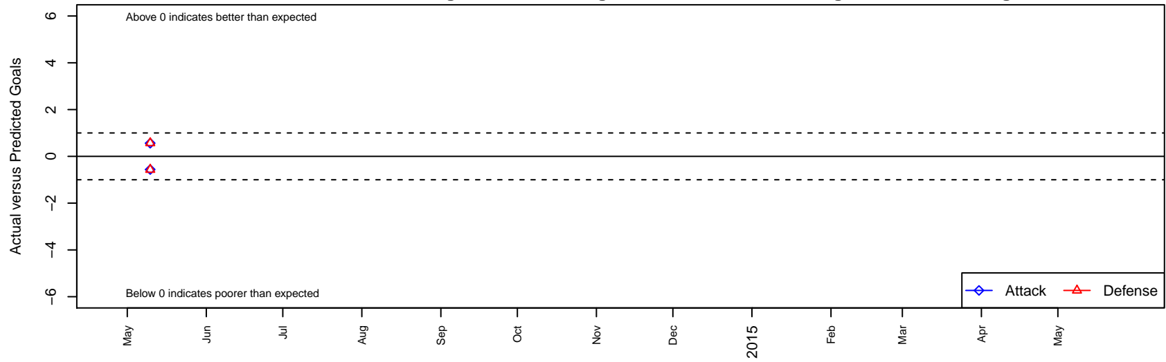
HYSA Arsenal B00 Dots are actual minus expected GF (blue circles) and GA (red triangles). Blue line is smoothed change in attack strength. Red is smoothed change in defense strength.
